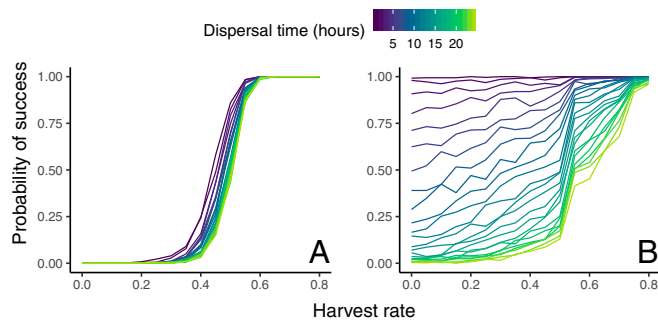
Fig. 1. Model predictions for management success. (A) Probability of successfully keeping the population to less than 300 individuals after 6 generations for different harvest rates and lengths of dispersal. (B) Probability of successfully preventing an invader from moving beyond patch 3 (of 6 total) after 6 generations for different harvest rates and lengths of dispersal. The curves are not smooth because the results come from stochastic simulations.
